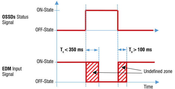
FIG. 30: EDM INPUT SIGNAL TIMING DIAGRAM
