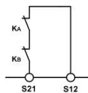
Fig. 9: Feedback loop for automatic start: The feedback loop monitors contactors or the expansion modules.
