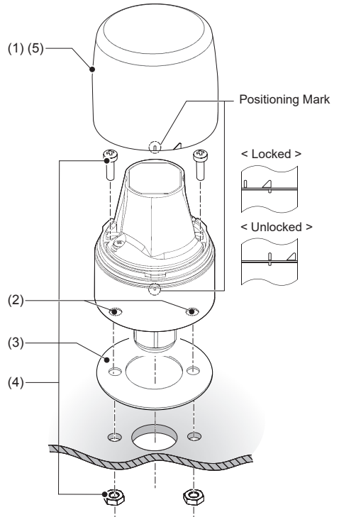
Installation Example
