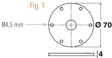
FOH - FSH 6 holes on Ø60 mm
